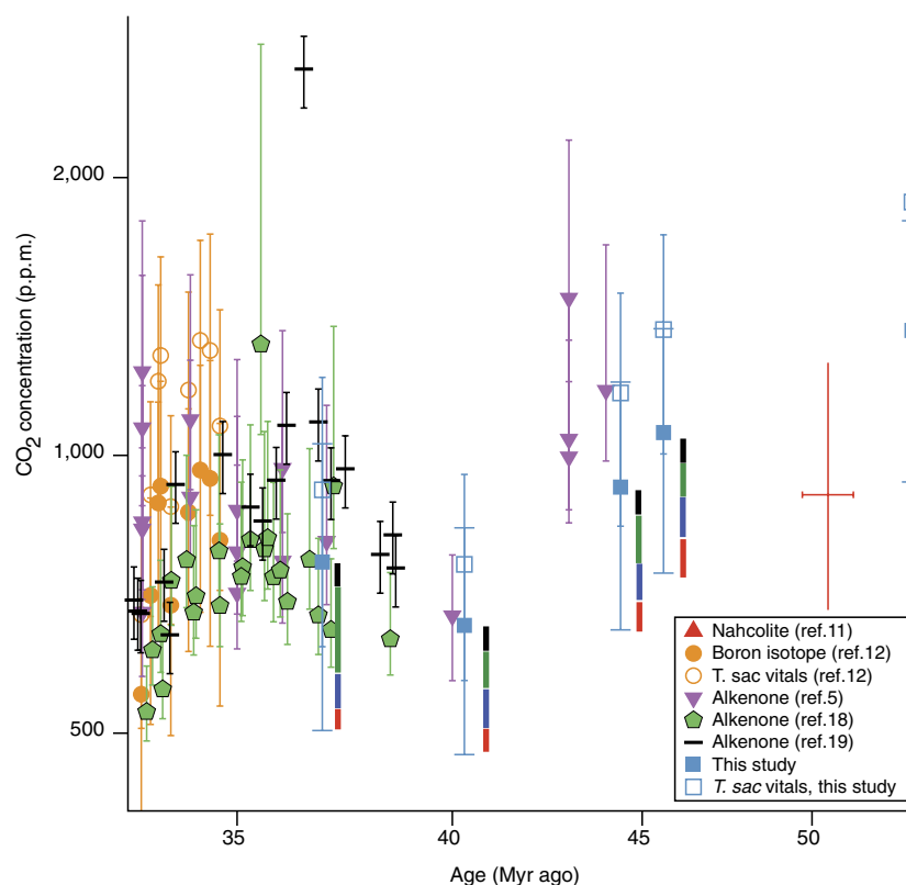
Extended Data Figure 4 | Compilation of several CO 2 records for the Eocene in comparison to this study. Data are from refs 5, 11, 12, 18 and 19. The contribution of different parameters to the uncertainty on our CO 2 reconstructions is colour-coded; sequentially from bottom to top, red is from \delta^{11}\text{B}_{\text{sw}} , blue is from the \Omega_{\text{calc}} uncertainty, green is from the \delta^{11}\text{B}_{\text{c}} error, black is the 40 p.p.m. uncertainty in the event of disequilibrium with the atmosphere. Other parameters contribute <10% uncertainty to the CO 2 calculations and are not shown. Note that the data from Pearson
