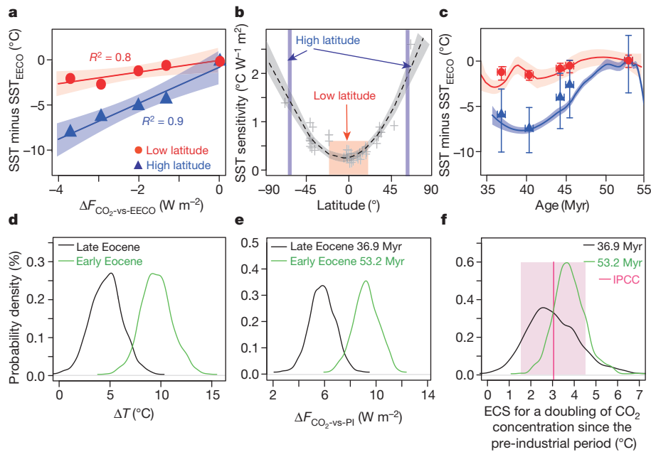
Figure 4 | CO 2 as a driver of latitudinal cooling in the Eocene, and ECS analyses of the EECO and late Eocene time slices. a , Evolving relationship between SST 14 for high and low latitudes and the CO 2 forcing of each of our time slices relative to the EECO, with linear regression fits and coefficients of determination ( R^2 ). b , Apparent latitudinal SST sensitivity for the last 520 kyr (ref. 13). The dashed line is the second-order polynomial through the SST sensitivity data (grey crosses) of ref. 13. Red shading shows the SST sensitivity estimates averaged as a low-latitude mean, and blue lines show the high-latitude mean. c , Reconstructed (lines) and estimated (symbols) SST relative to 53.2 Myr ago. Symbols are estimated using the respective CO 2 reconstructions and the average low-latitude (red circles) and high-latitude (blue triangles) SST
