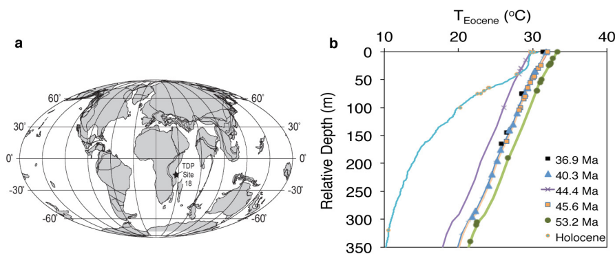
Extended Data Figure 1 | Palaeogeography and \delta^{18}\text{O} -derived temperature against foraminiferal calcification depth. a , Approximate palaeoposition of Tanzanian Drilling Project (TDP) sites studied here (map generated from www.ods.n.de ). b , Reconstructed temperature ( T_{\text{Eocene}} ) and relative depth of each foraminifera within each time slice. The pale blue line represents the output of a General Circulation Model simulation run with Eocene boundary conditions 89,90 , whereas the other coloured lines show the General Circulation Model output offset to intersect with the warmest temperature at
