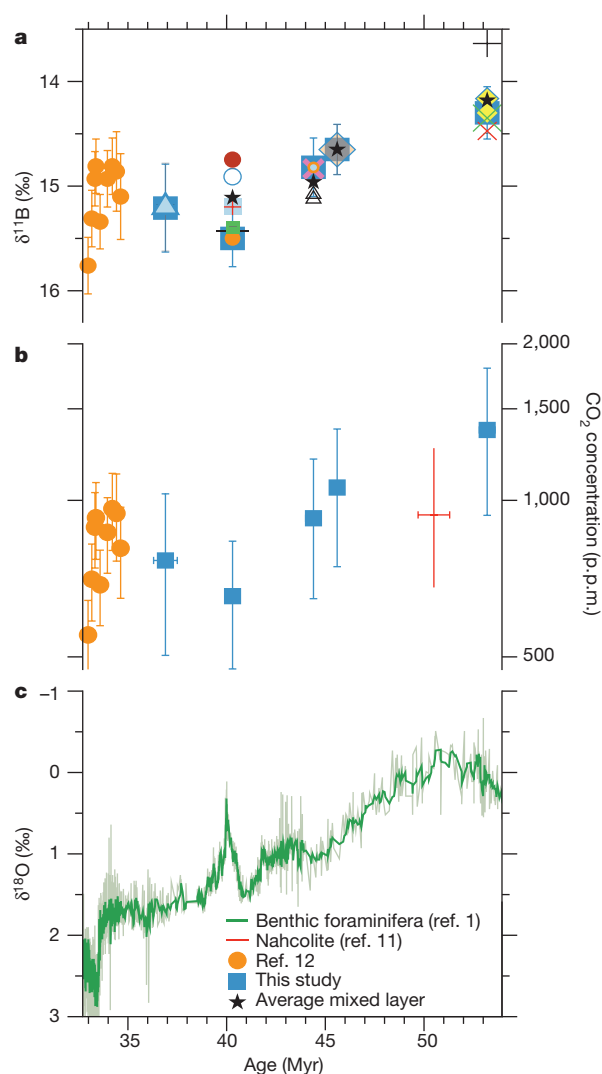
Figure 3 | New atmospheric \text{CO}_2 reconstructions from shallow planktonic foraminiferal \delta^{11}\text{B} . a , \delta^{11}\text{B} of shallower foraminifera (symbols as in blue-shaded areas of Fig. 2) and asterisks represent the average of those for each time slice. Blue squares and orange circles represent the warmest species used in b . Ref. 12 data are offset (Supplementary Table 2, Methods). b , Atmospheric \text{CO}_2 assuming \delta^{11}\text{B}_c = \delta^{11}\text{B}_{\text{borate}} using the warmest species of each time slice. The red line is based on ref. 11. c , Benthic foraminiferal \delta^{18}\text{O} (ref. 1) (as in Fig. 1b). Age error bars ( b ) are based on the ages of the nearest datums, \delta^{11}\text{B} errors are as in Fig. 2, and the \text{CO}_2 uncertainty is based on the 95% confidence of Monte Carlo error propagation (Methods).
