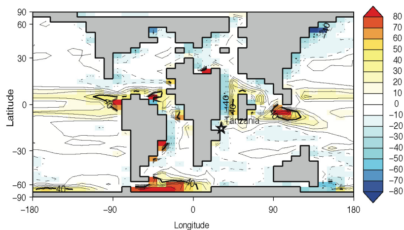
Extended Data Figure 6 | The cGENIE estimates of air-seawater \text{CO}_2 disequilibrium. The colour scale shows the difference between \text{pCO}_2 in air and \text{pCO}_2 in sea water. The model uses Eocene boundary conditions and positive values mean that seawater is a source of \text{CO}_2 (in parts per million); the star shows the palaeo-location of Tanzania.
