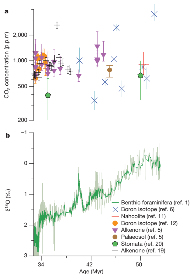
Figure 1 | Currently available Eocene atmospheric CO 2 records and benthic foraminiferal \delta^{18}\text{O} values. a , CO 2 reconstructions 5,6,11,12,19,20 with the 2 s.d. uncertainties. b , Benthic foraminiferal \delta^{18}\text{O} (ref. 1). The green line shows the five-point moving average of the grey line, with data age modified to account for the revised timing of the MECO 30 . Lower benthic \delta^{18}\text{O} values denote warmer bottom-water temperatures (or less ice volume, which is assumed to be minimal in the Eocene). Error bars on \delta^{18}\text{O} are smaller than the symbols (Methods).
