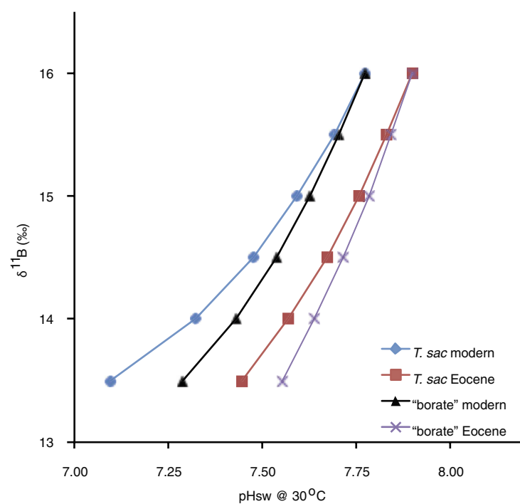
Extended Data Figure 9 | The effect of seawater composition on boron isotope calibrations in foraminifera. The example of T. sacculifer calibration 22 and the 'borate' calibration (assuming \delta^{11}\text{B}_c = \delta^{11}\text{B}_{\text{borate}} ) for modern and Eocene seawater compositions; see Methods and Supplementary Table 2.
