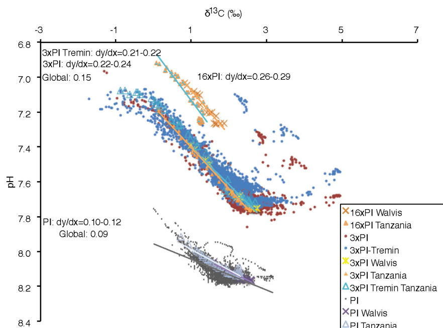
Extended Data Figure 10 | The cGENIE output of seawater pH versus \delta^{13}\text{C} for the top ~300 m of the ocean. The scenarios explored are from offshore Tanzania (triangles), Walvis Ridge in the South Atlantic Ocean (crosses), and the global ocean (circles) at three different atmospheric \text{CO}_2
