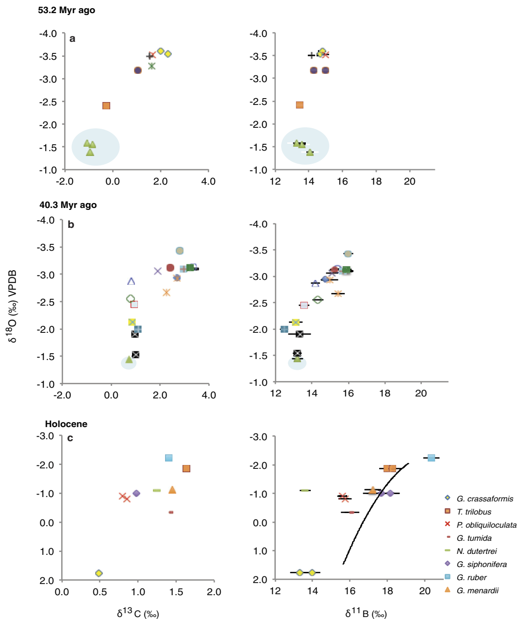
Extended Data Figure 7 | Comparison of Eocene and modern planktonic foraminiferal \delta^{11}\text{B} and \delta^{13}\text{C} with \delta^{18}\text{O} . a and b show analyses from the time slices 53.2 Myr ago and 40.3 Myr ago, respectively (as in Fig. 2 and Supplementary Table 1). Cibicidoides species ( Cibs ) are shaded in blue. c , Core-top (Holocene) offshore Tanzania foraminiferal measurements. Seawater \delta^{11}\text{B}_{\text{borate}} and \delta^{18}\text{O} was calculated from temperature, alkalinity and dissolved inorganic carbon measurements
