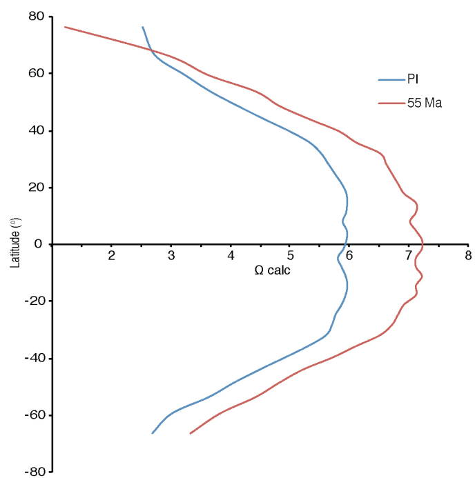
Extended Data Figure 3 | cGENIE estimates of calcite saturation in surface waters. Comparison of calcite saturation \Omega_{\text{calc}} for pre-industrial times (PI; blue) and 55 Myr ago (red) at different latitudes.
