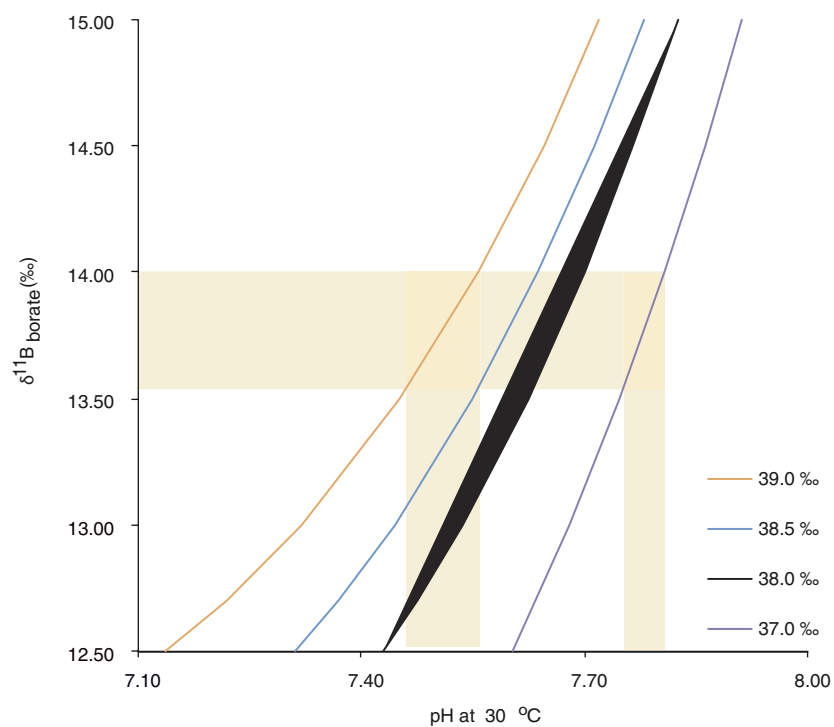
Extended Data Figure 2 | \delta^{11}\text{B} versus pH as a function of \delta^{11}\text{B}_{\text{sw}} . Increasing \delta^{11}\text{B}_{\text{sw}} , as indicated for each line in units of per mil, results in lower pH for the same \delta^{11}\text{B} . However, for the same \delta^{11}\text{B} range, the reconstructed pH range is larger for higher \delta^{11}\text{B}_{\text{sw}} (see brown-shaded regions).
