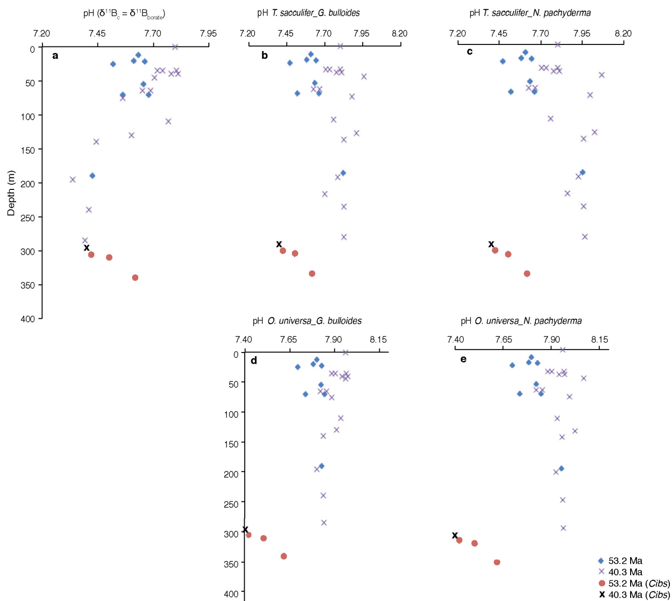
Extended Data Figure 8 | Reconstructed pH using different combinations of published symbiont-bearing and non-symbiotic foraminiferal vital-effect calibrations for the two most complete with depth time slices. a shows the case where no vital effect corrections were applied for comparison. The vital-effect corrections for deeper asymbiotic planktonic foraminifera are based on either Globigerina bulloides 26 (b and d) and Neoglobobulimina pachyderma 65 (c and e) calibrations.
